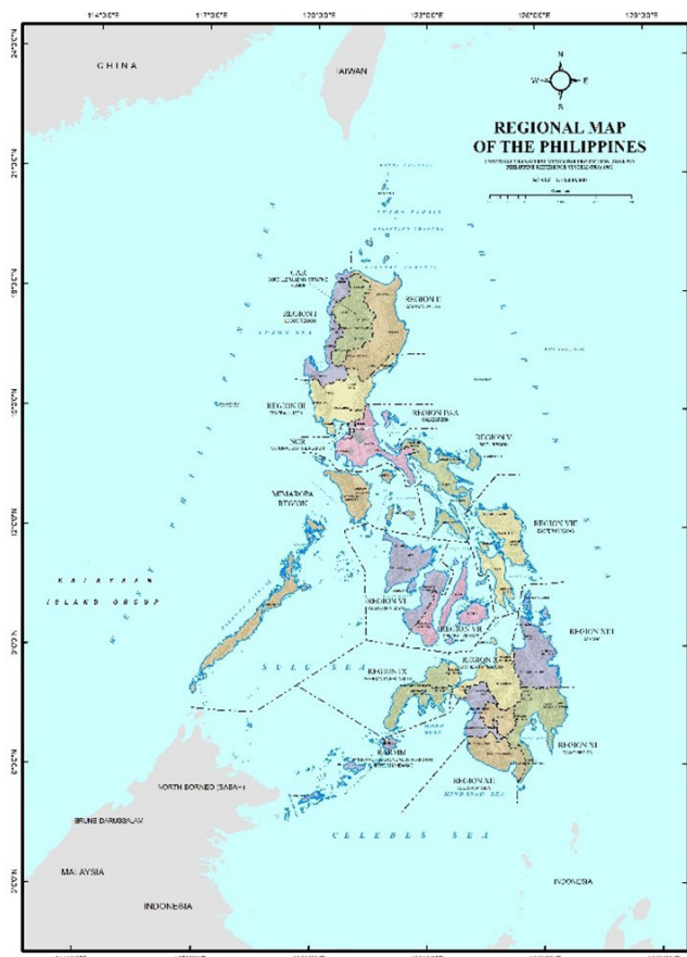
Figure 2.1.1 Location map
