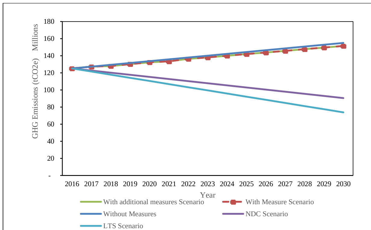
Figure II. 9: Projections of greenhouse gas emissions and removals under different scenarios
