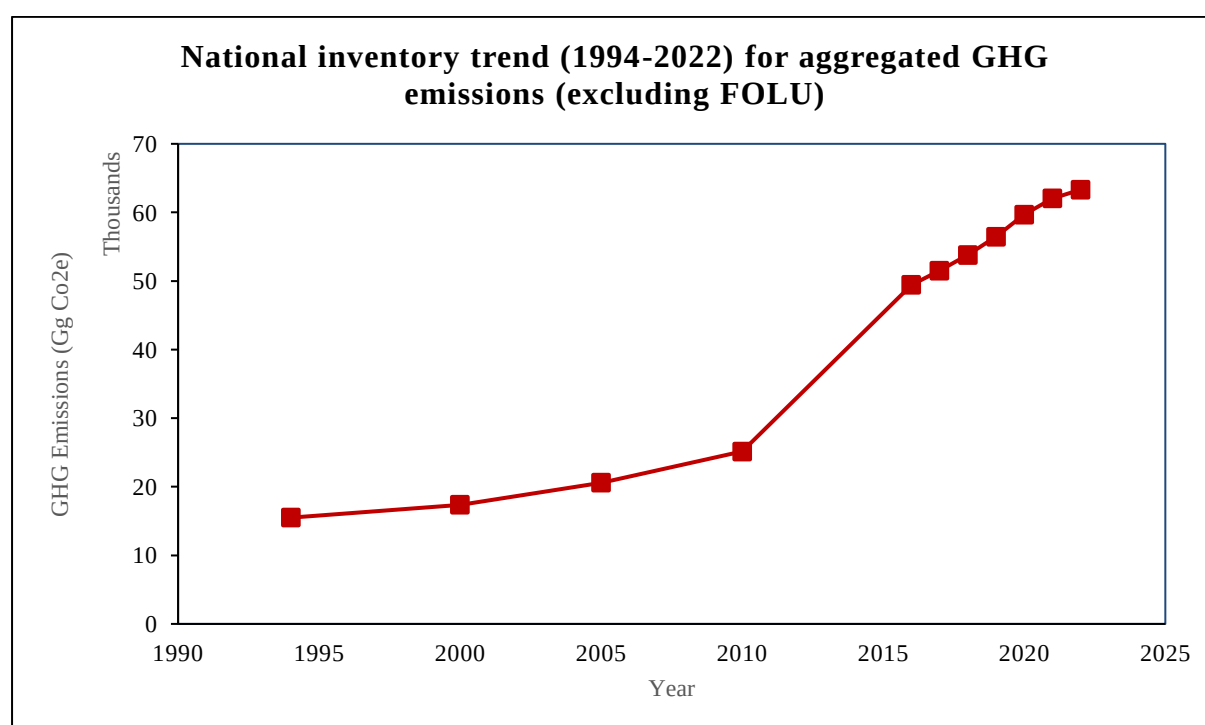
Figure I. 21: National inventory trend (1994-2022) for aggregated GHG emissions (Excluding FOLU)
