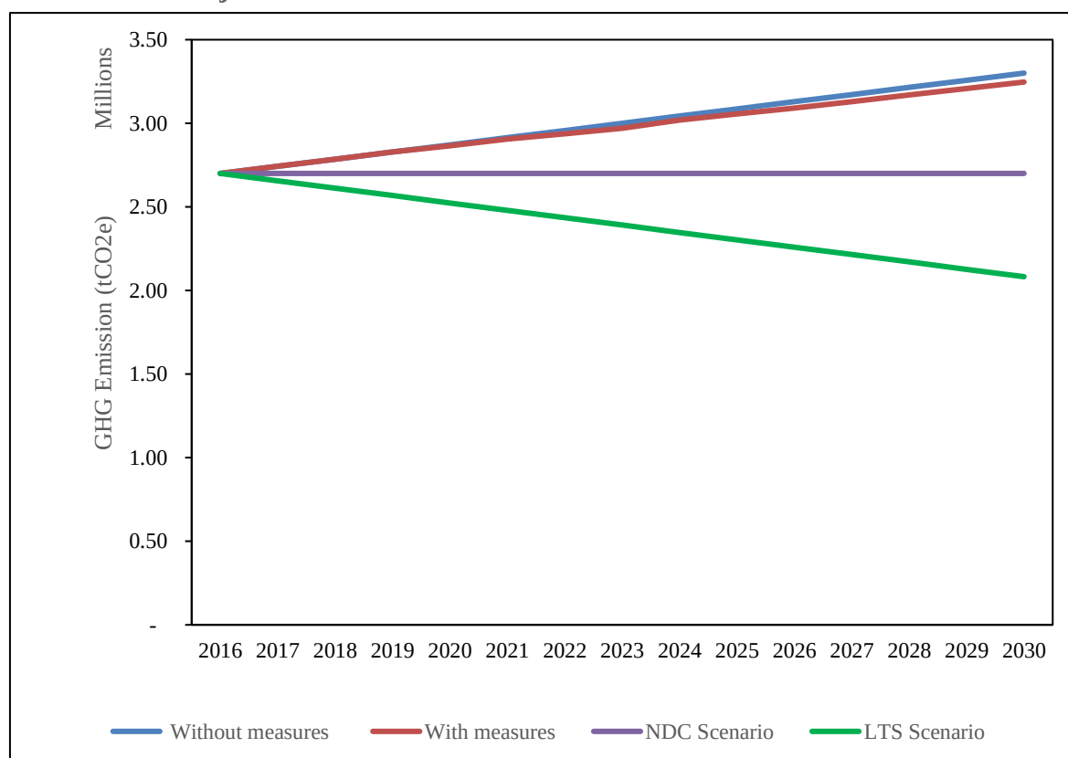
Figure II. 11: Projections of greenhouse gas emissions and removals under different scenarios- Waste sector
