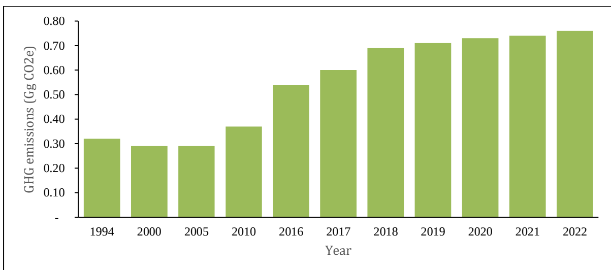
Figure I. 28: N 2 O emission trend in the energy sector of Cambodia (1994-2022)
