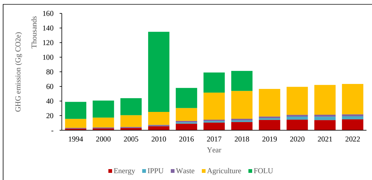
Figure I. 23: Trend in total emissions by sector from 1994 to 2022
