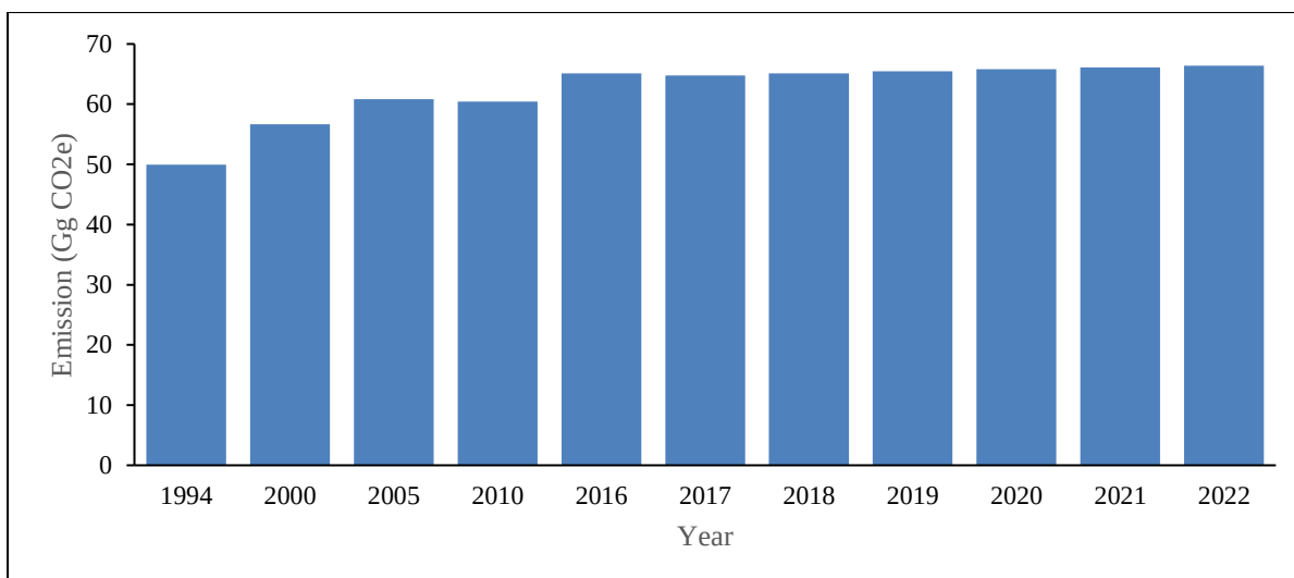
Figure I. 38: CO 2 emissions under the waste sector In Cambodia for 1994-2022
