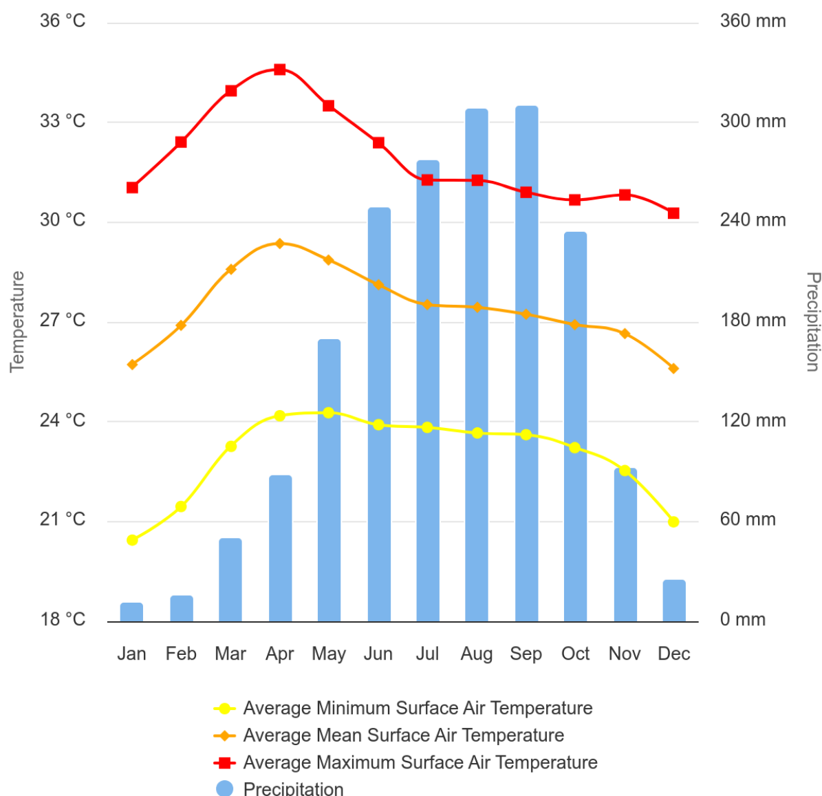
Figure I. 2: Monthly Climatology of Average Minimum Surface Air Temperature, Average Mean Surface Air Temperature, Average Maximum Surface Air Temperature & Precipitation 1991-2020; Cambodia
