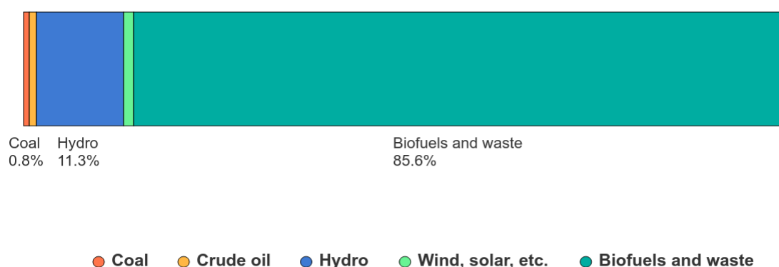
Figure I. 45: The domestic energy production in Cambodia in 2021
