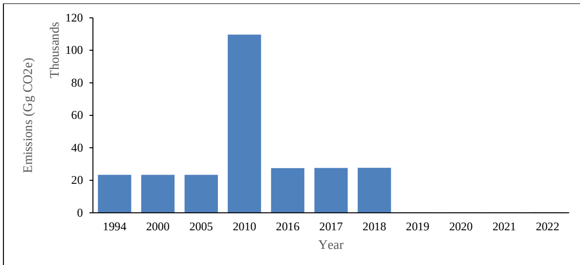
Figure I. 34: CO 2 emission trend in AFOLU sector in Cambodia (1994-2022)
