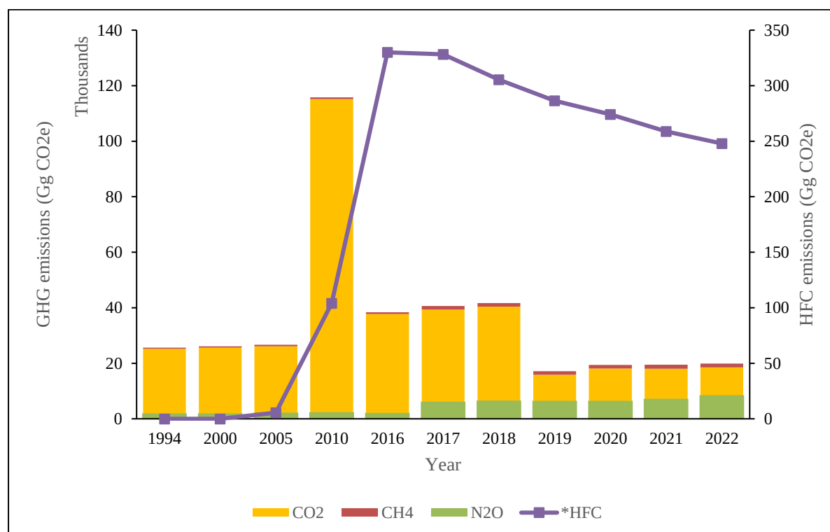
Figure I. 24: Trend in GHG emissions by gas type, 1994-2022
